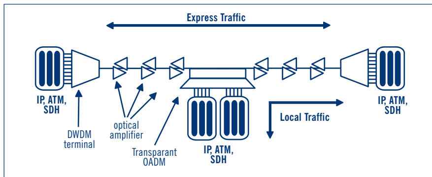
Figure 1. Optical transmission system architecture
