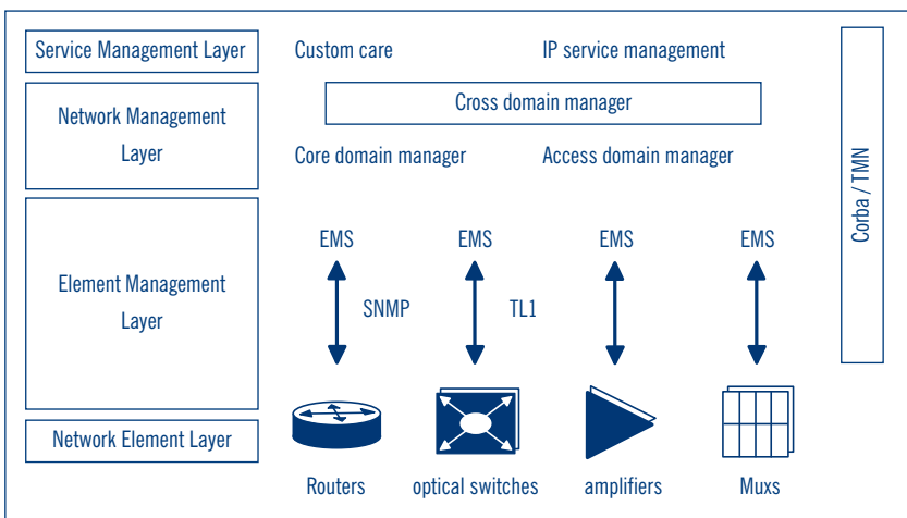
Figure 3. A typical TMN architecture
