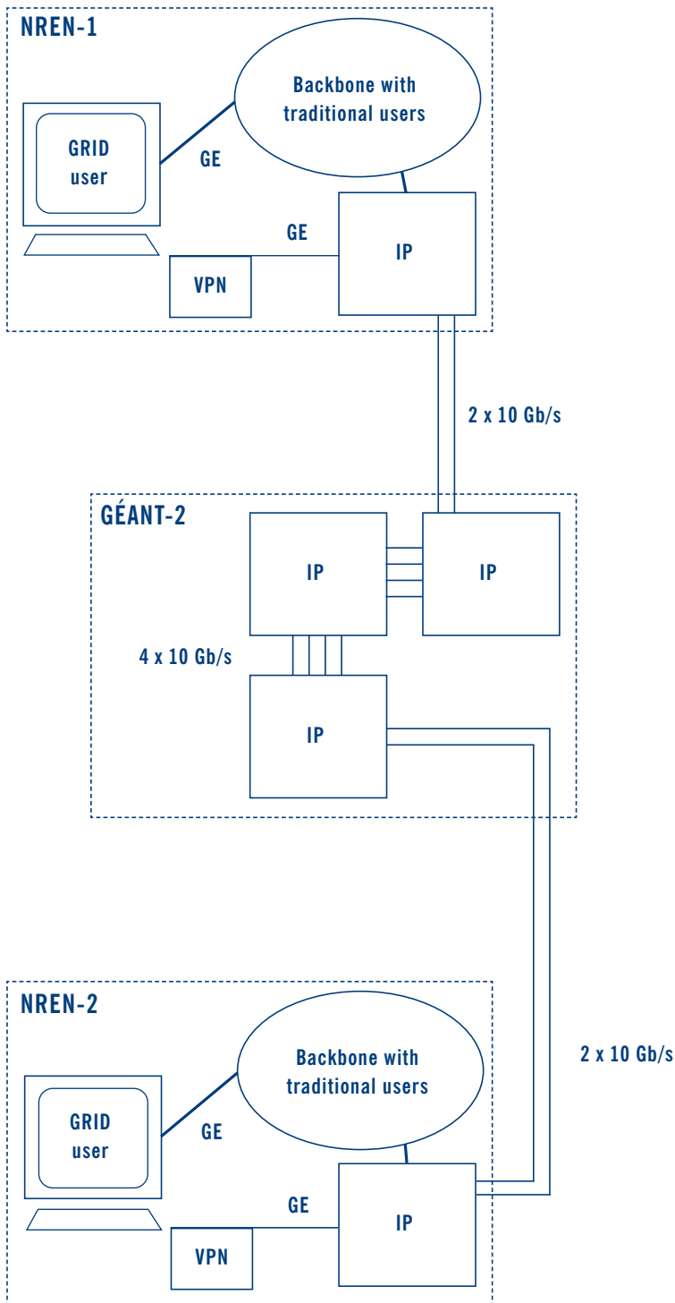
Figure 6. Shared IP-only network architecture
