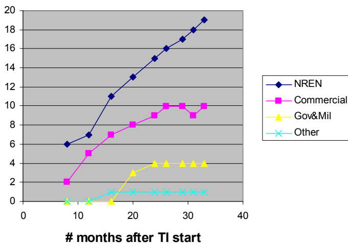
# "Accredited" CSIRTs
