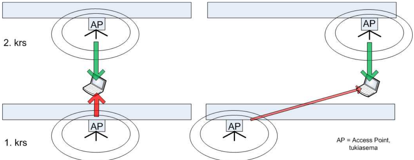
Figure 1. Interference between access points. If access points are placed directly above or below each other, their signals interfere with each other (left). If the access points are located in slightly different places on different floors, the interfering signal fades as it travels through the ceiling, resulting in less interference (right).
